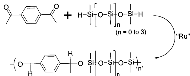
Figure 1. Ru-catalyzed hydrosilylation copolymerization.
